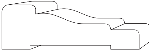
BLC 129 3/4" x 2 1/4"
