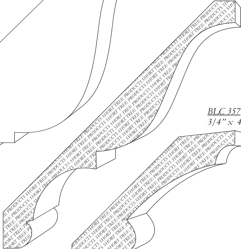
BLC 356 3/4" x 6"
