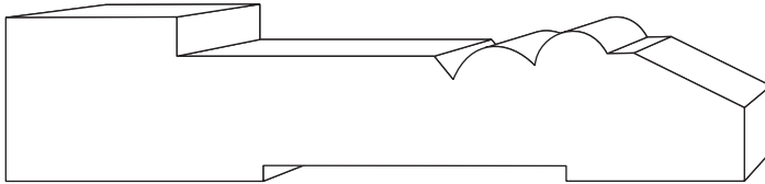
BLC 114 3/4" x 3 1/2"
