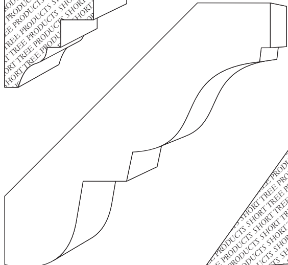
BLC 360 3/4" x 3 3/4"
