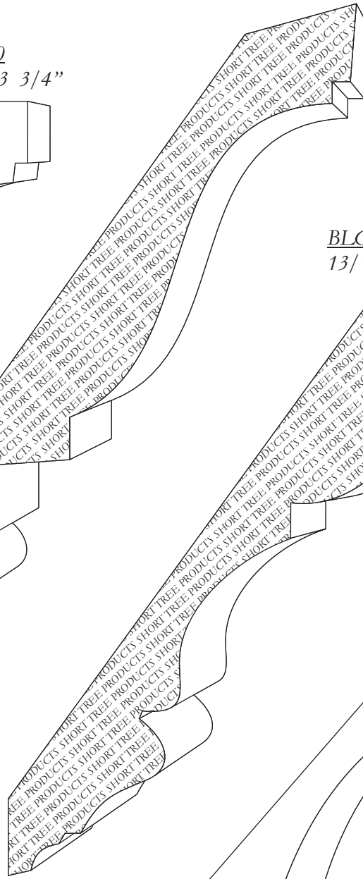
BLC CR-860 13/16" x 7"
