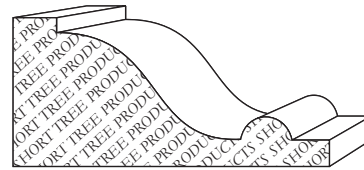
BLC 614 3/4" x 1 5/8"
