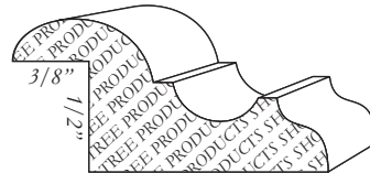
*BLC 617 11/16" x 1 1/2"
